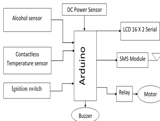
Fig. 1. Block diagram of the proposed alcohol and temperature monitoring system
