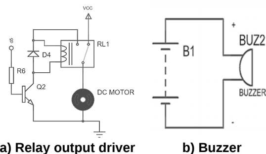
Fig. 6. The relay output driver and buzzer unit (Jha, 2016)
