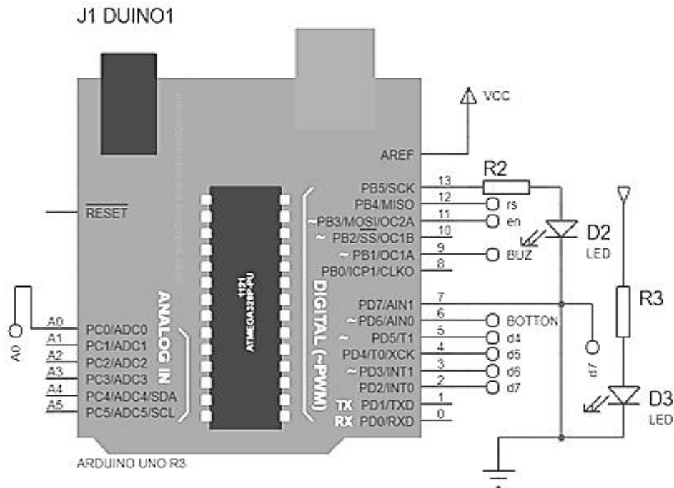
Fig. 7 Microcontroller unit (Ojha et al., 2016)
