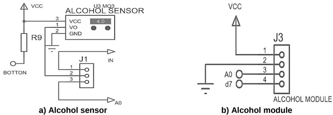
Fig. 2. Alcohol sensor and module (Jha, 2016)
