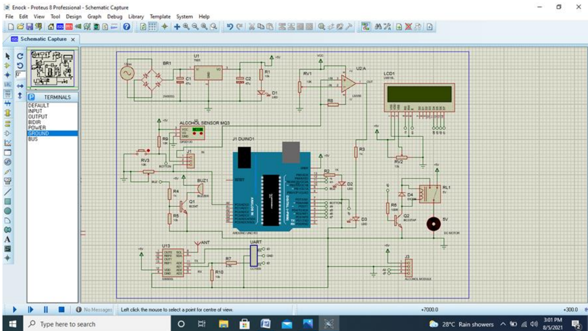
Fig. 10. Simulated general circuit
