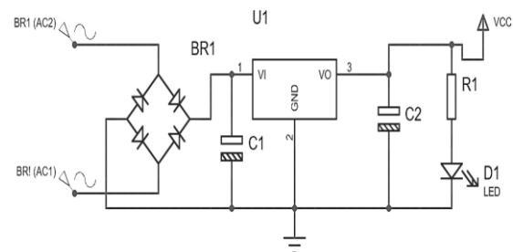
Fig. 8 Regulated power supply unit (Eugene, 2018)
